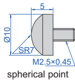
spherical point
