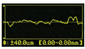
roughness profile
